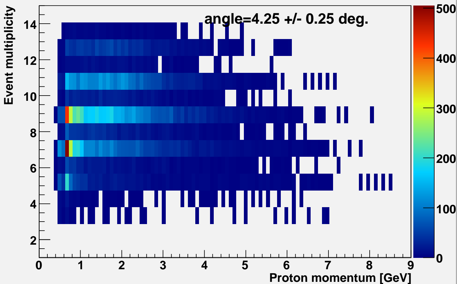
Event multiplicity vs p-momentum alpha=4.25
