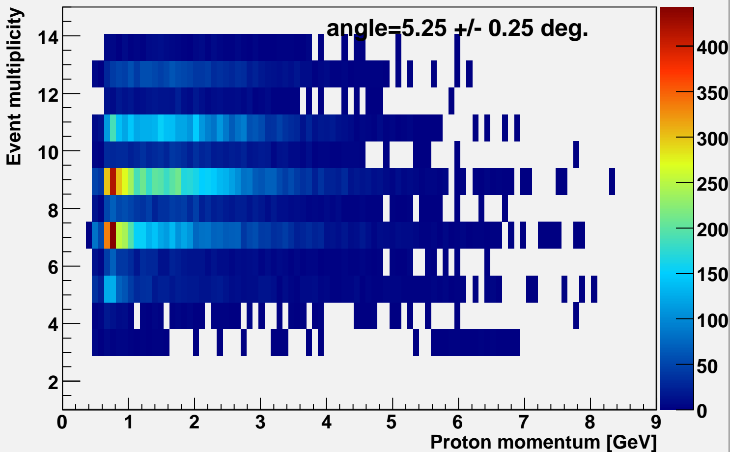
Event multiplicity vs p-momentum alpha=5.25
