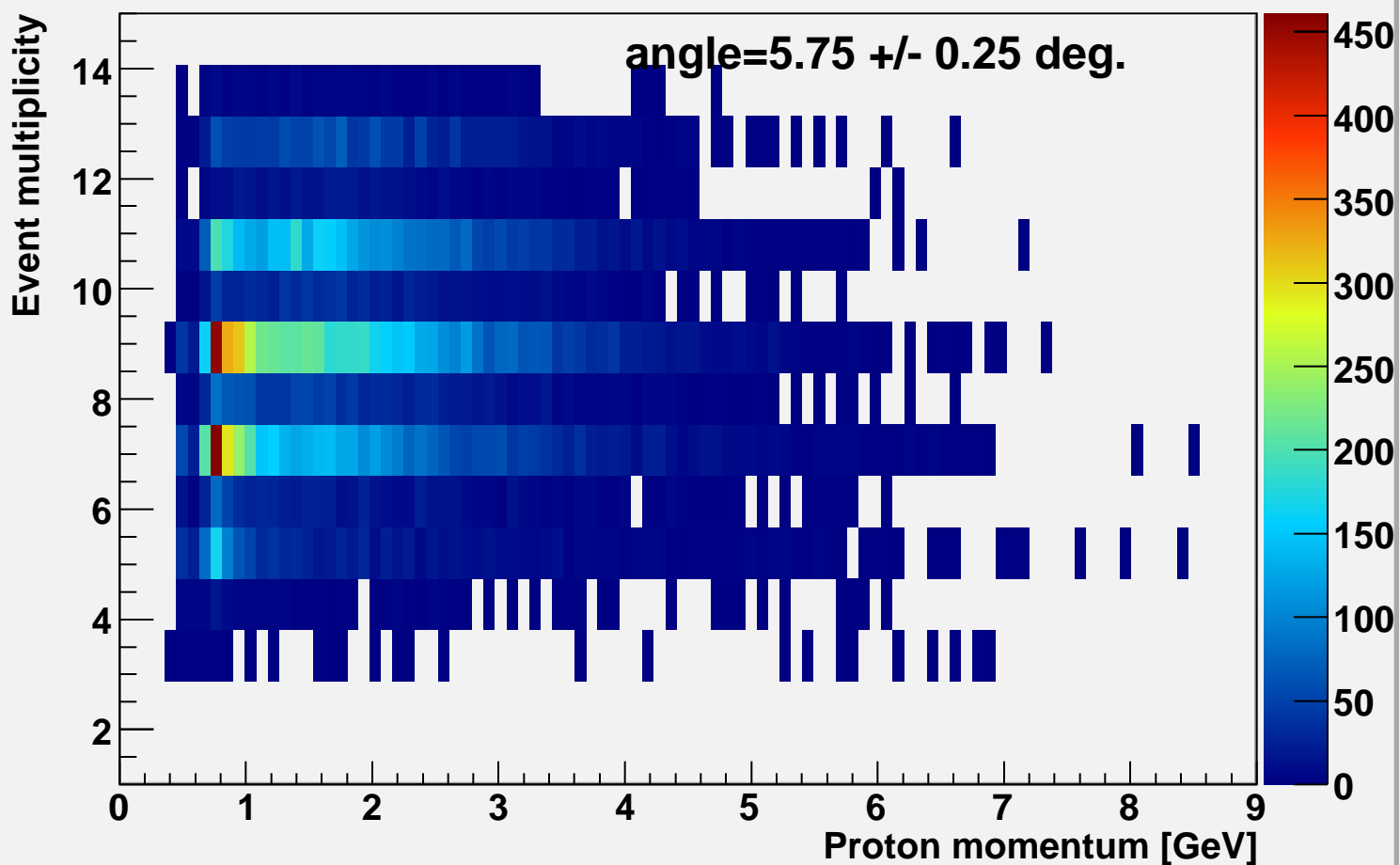
Event multiplicity vs p-momentum alpha=5.75
