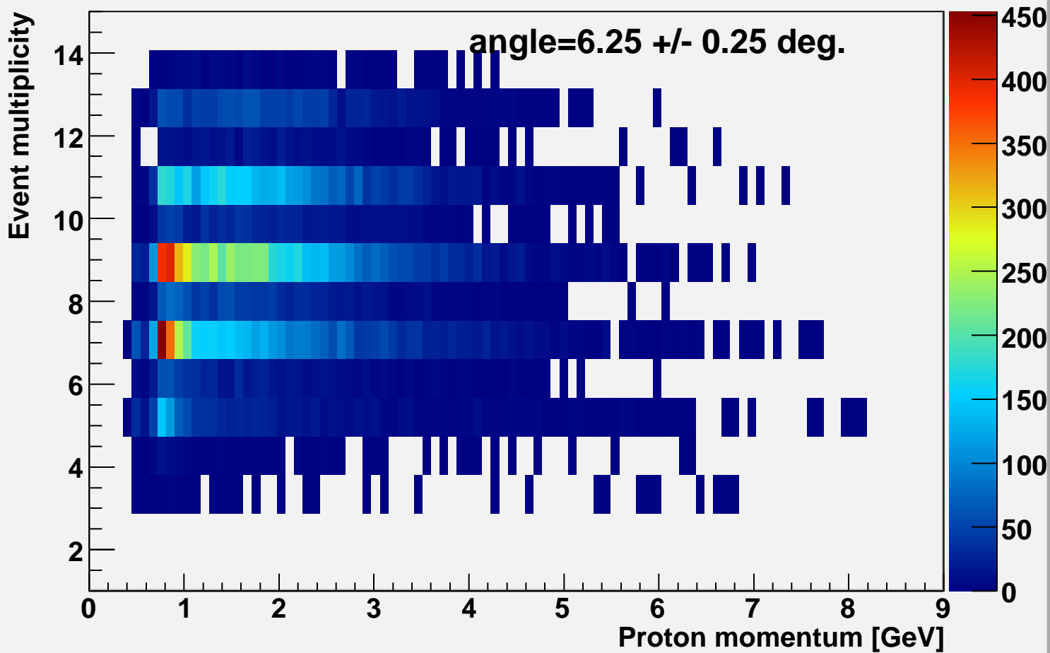
Event multiplicity vs p-momentum alpha=6.25
