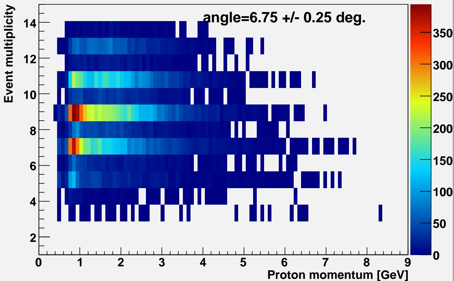
Event multiplicity vs p-momentum alpha=6.75
