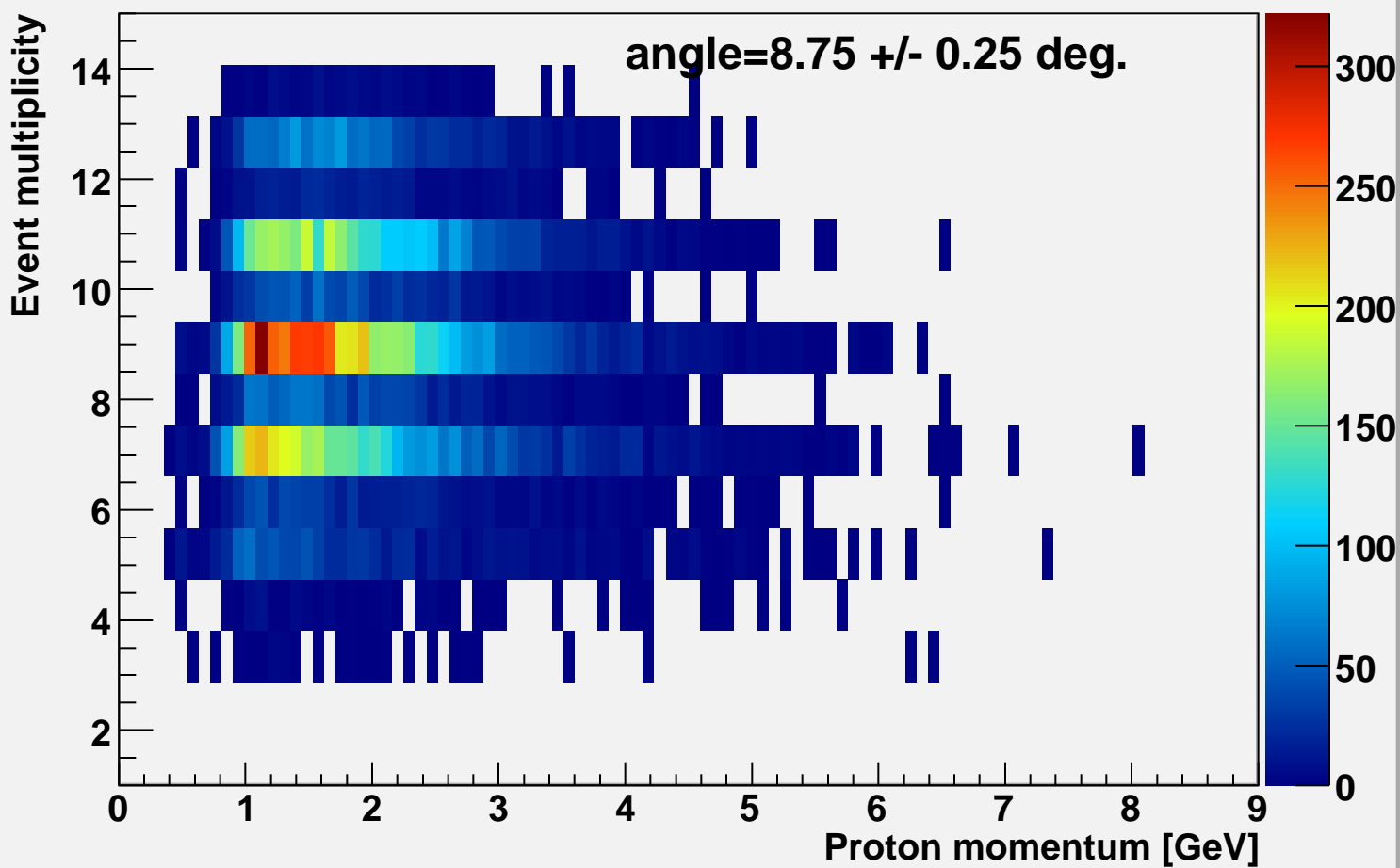
Event multiplicity vs p-momentum alpha=8.75
