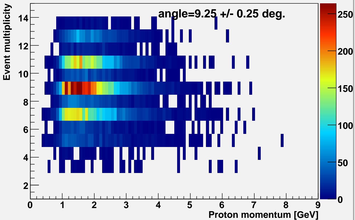
Event multiplicity vs p-momentum alpha=9.25
