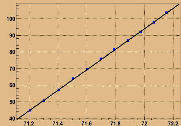
Break Down Volatage = 70.48
