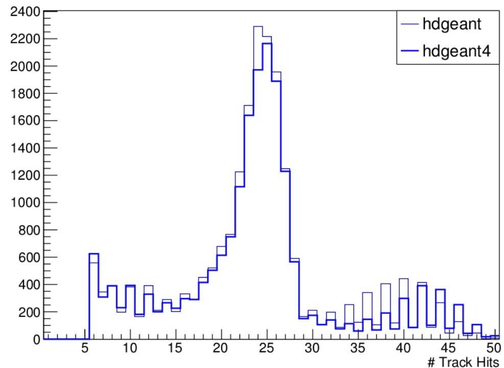
/Independent/Hist_Reconstruction/Tracking/NumDCHitsPerTrack
