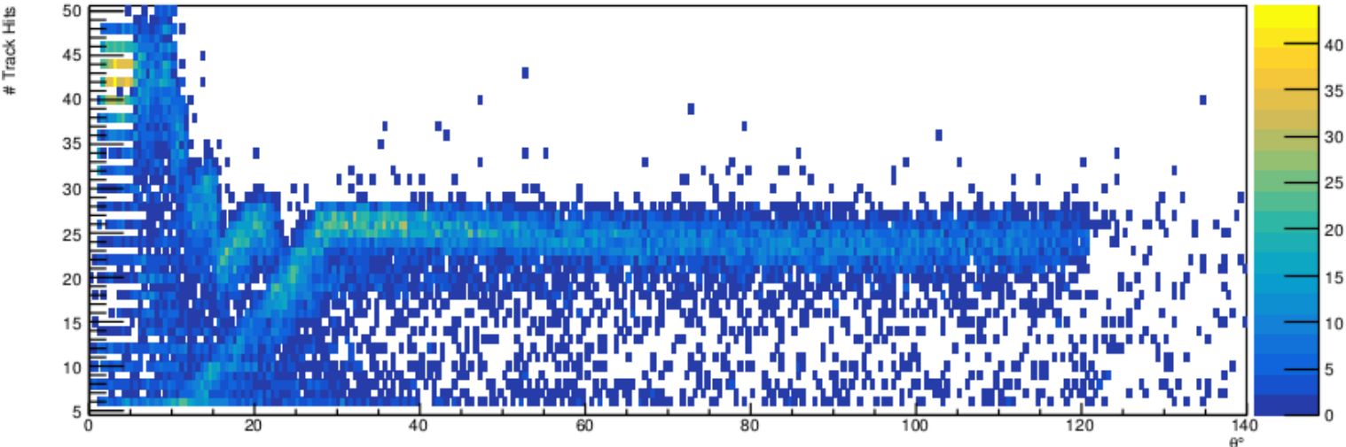
/Independent/Hist_Reconstruction/Tracking/NumDCHitsPerTrackVsTheta - HG4
