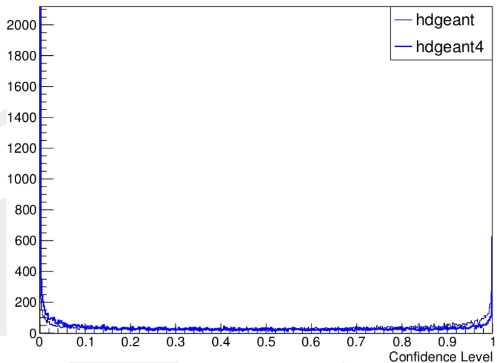
/Independent/Hist_Reconstruction/Tracking/TrackingFOM
