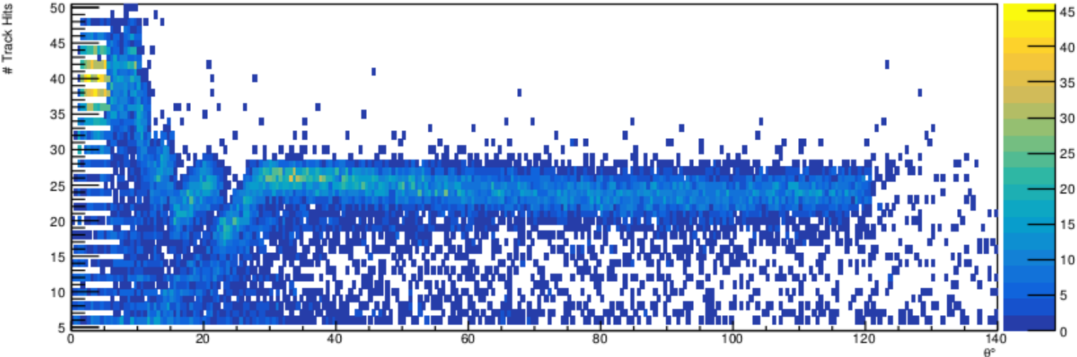
/Independent/Hist_Reconstruction/Tracking/NumDCHitsPerTrackVsTheta - HG3
