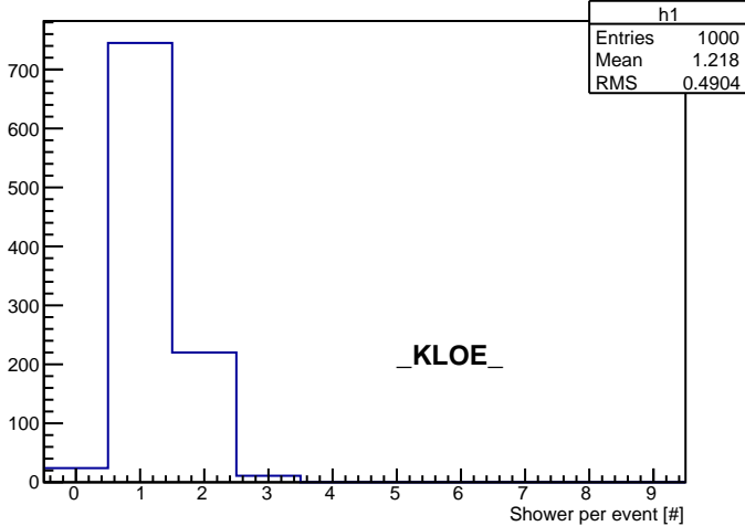
Gamma Multiplicity
