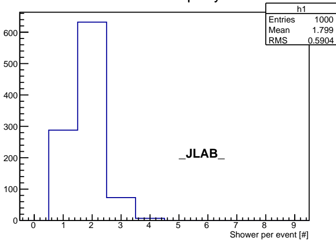
Gamma Multiplicity
