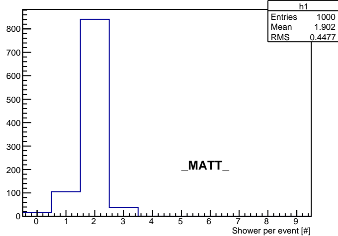
Gamma Multiplicity
