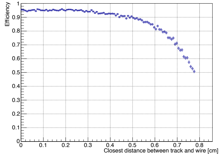
CDC Per Straw Efficiency Vs. DOCA
