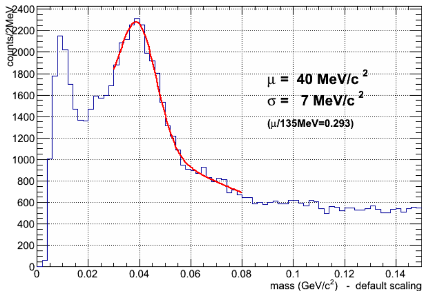
2 \gamma inv. mass (UNSCALED)
