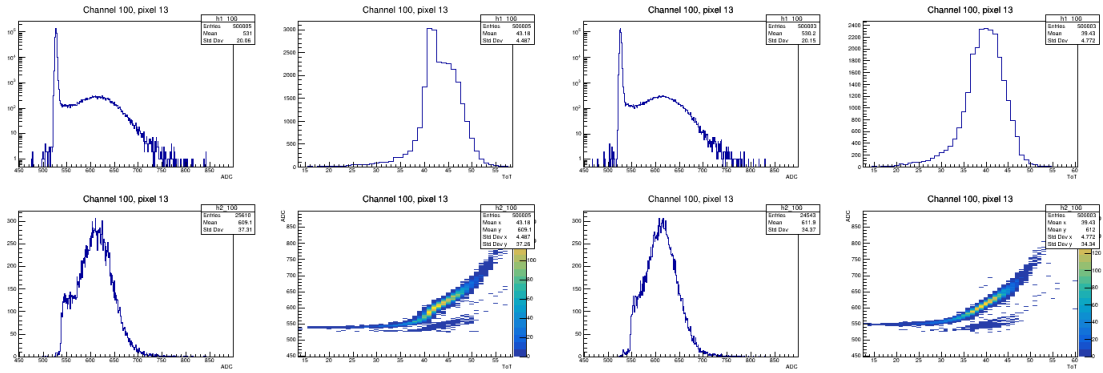
Figure 1: Effect of TDC Threshold cuts (THR = 50 left, THR = 100 right) on Time over Threshold
