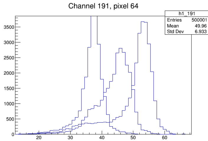
Figure 2: Time of threshold distributions for gain = 32, 64, and 128 from laser test data.
