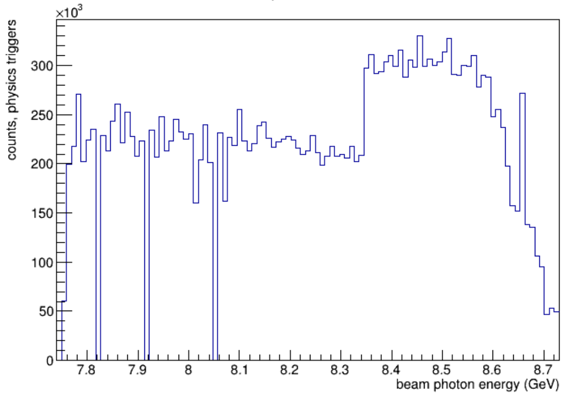
run 71724, all DBeamPhoton
