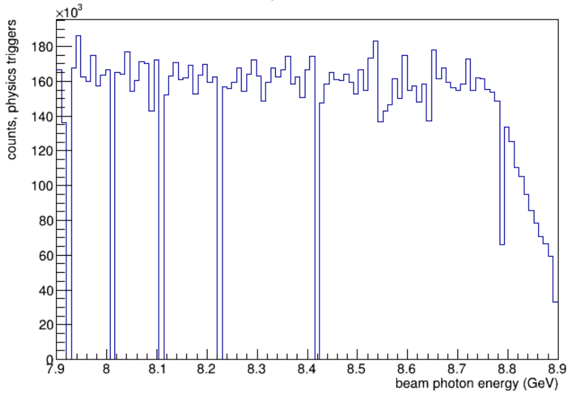
run 51768, all DBeamPhoton
