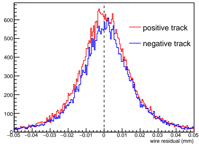
plane 24 (wire)
