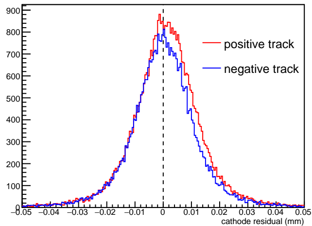
plane 24 (cathode)
