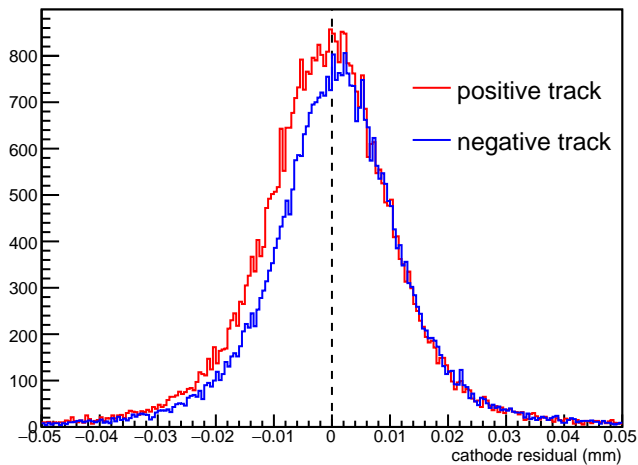
plane 21 (cathode)
