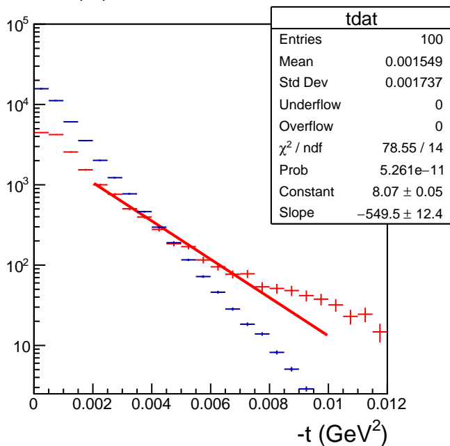
twopi_primakoff_DSelect_test_W_100000
