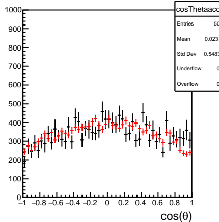
twopi_primakoff_DSelect_test_W_100000
