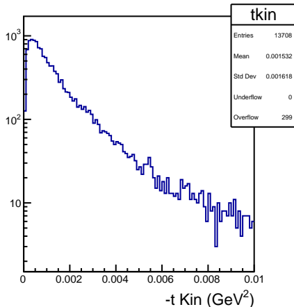
DSelector_Z2pi0_trees_test_signal_100000
