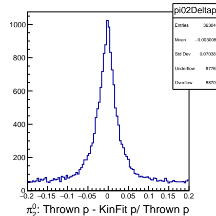
DSelector_Z2pi0_trees_test_signal_100000
