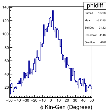
DSelector_Z2pi0_trees_test_signal_100000
