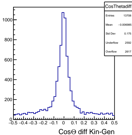
DSelector_Z2pi0_trees_test_signal_100000
