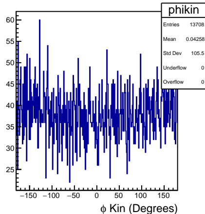
DSelector_Z2pi0_trees_test_signal_100000
