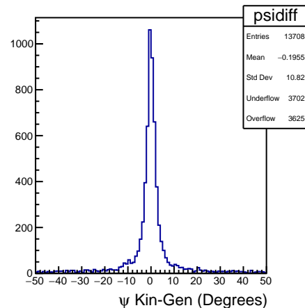
DSelector_Z2pi0_trees_test_signal_100000
