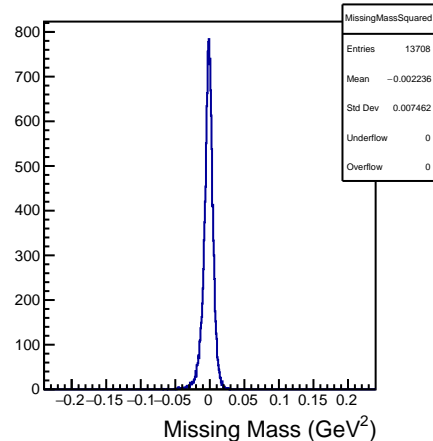
DSelector_Z2pi0_trees_test_signal_100000
