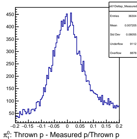
DSelector_Z2pi0_trees_test_signal_100000
