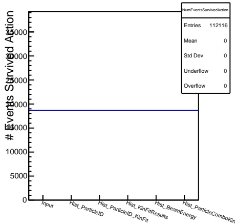
DSelector_Z2pi0_trees_test_signal_100000
