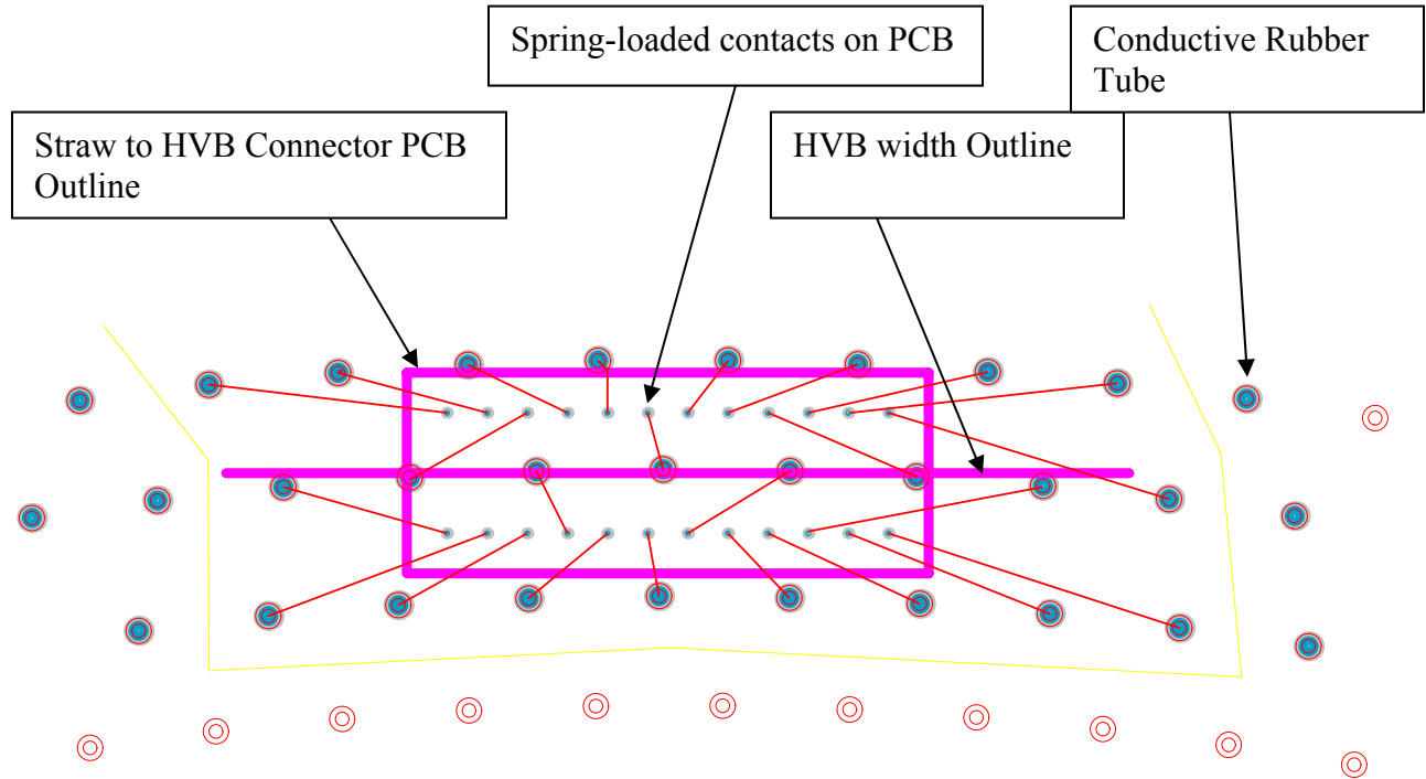
Routing on Layers 26, 27 and 28 – 24 channels.
