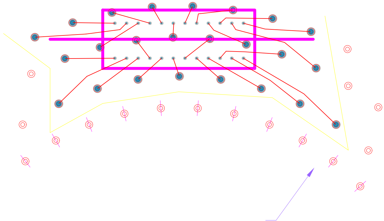
Routing on Layers 2, 3 and 4 – 24 channels.
