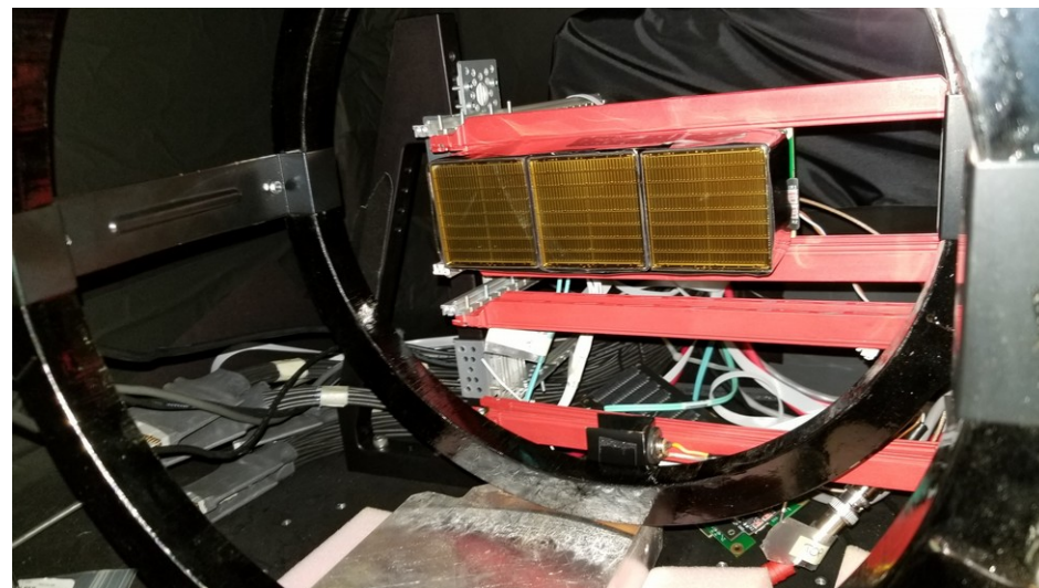
Shielding around the whole module and center PMT
