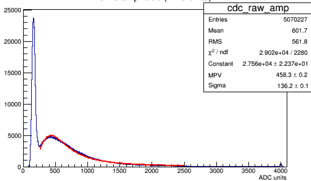
CDC amplitude (ADC units)
