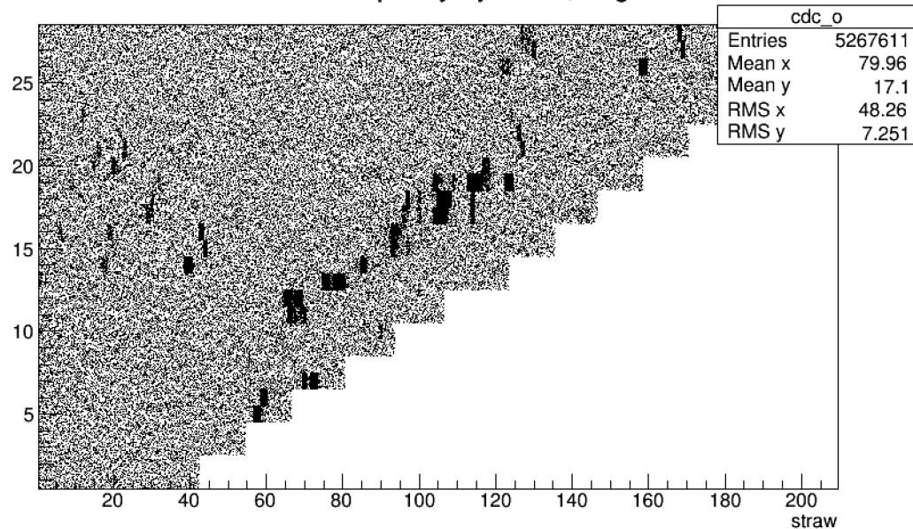
CDC occupancy by straw, ring
