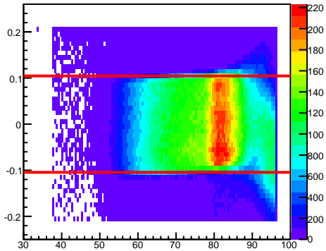
SC Match \Delta \phi - Sector 21
