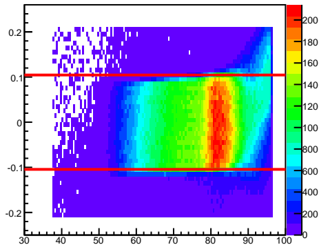
SC Match \Delta \phi - Sector 10
