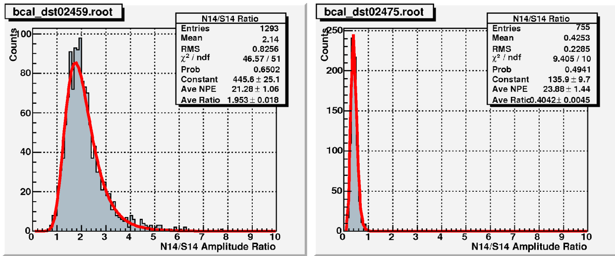
Figure 13: Typical ratio spectra in the run 2459 (left panel) and in the run 2475 (right panel). The red lines are the fits to the spectra (see Eq. 3).
