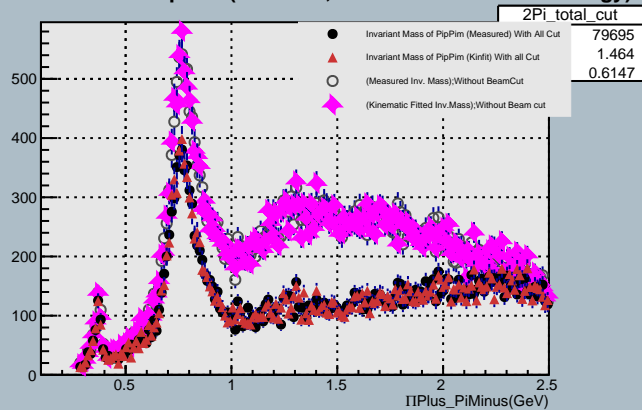
Invariant Mass of PipPim:(Total cut, Without cut on BeamEnergy)
