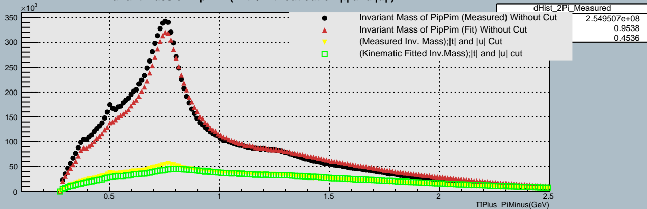
Invariant Mass of PipPim:(With/Without cut on |t| and |u| )
