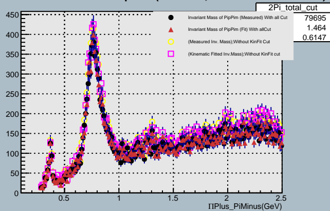
Invariant Mass of PipPim:(Total cut, Without cut on KinFit)
