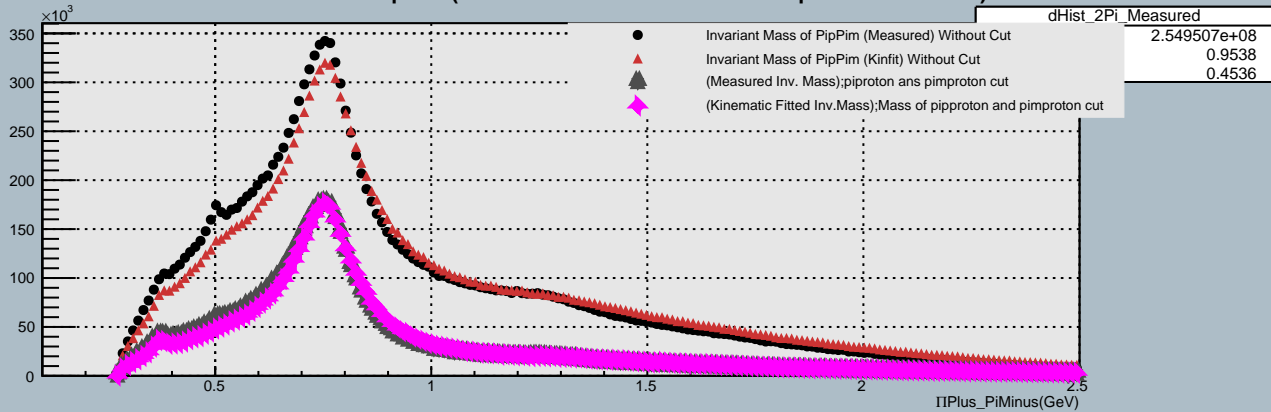
Invariant Mass of PipPim:(With/Without cut on masses of PipProt && PimProt)
