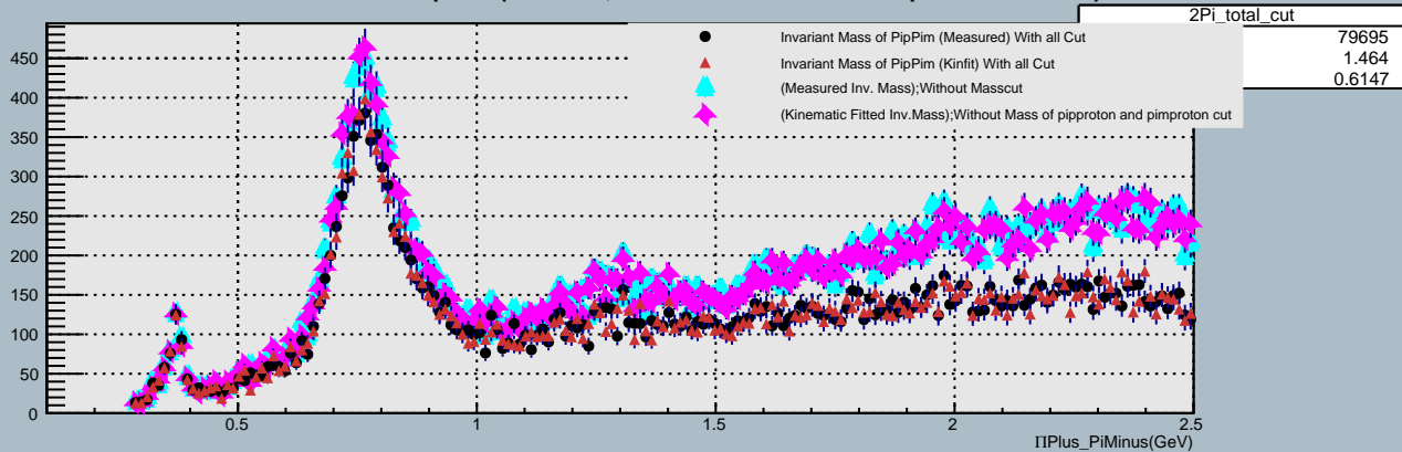
Invariant Mass of PipPim:(Total cut, Without cut on Mass of Piprot && PimProt)
