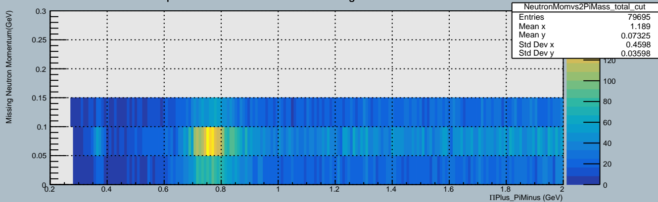
PiplusPiminus vs Momentum of Missing Neutron after all cut
