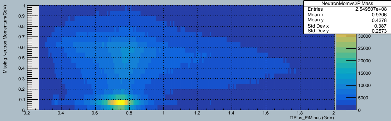
PiplusPiminus vs Momentum of Missing Neutron
