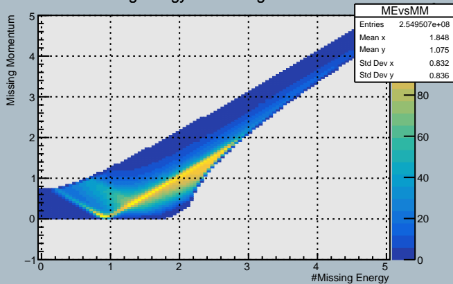
MissingEnergy vs MissingMomentum
