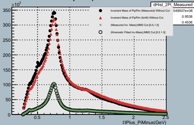
Invariant Mass of PipPim:(With/Without cut on MM2)
