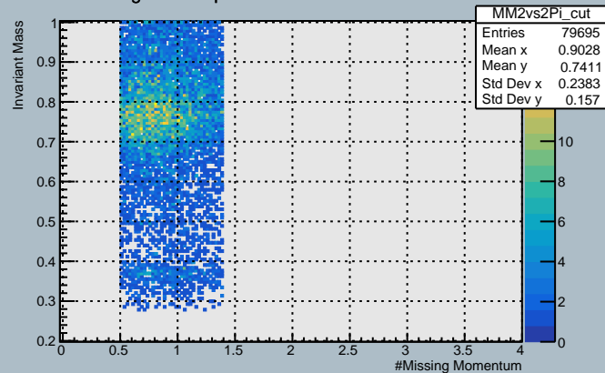
Missing Mass Square vs Invariant massAfter all cut
