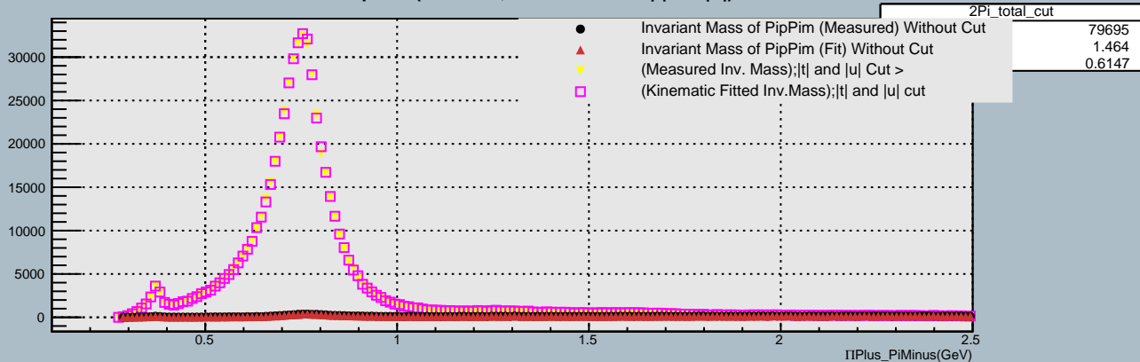
Invariant Mass of PipPim:(Total cut, Without cut on |t| && |u|)
