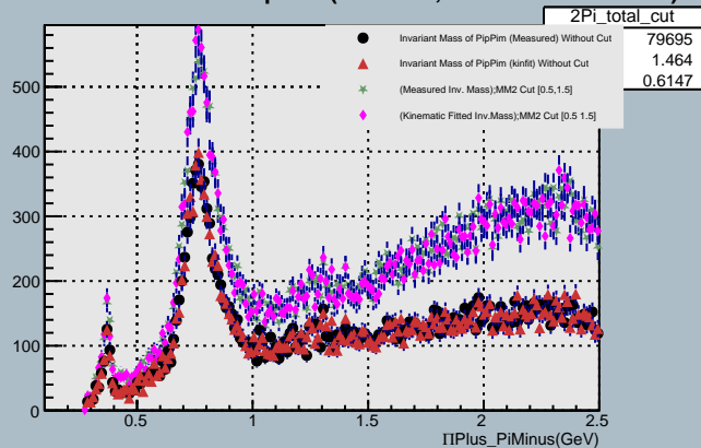
Invariant Mass of PipPim:(Total cut, Without cut on MM2)
