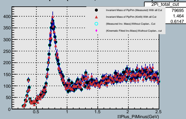
Invariant Mass of PipPim:(Total cut, Without cut on Coplanarity)
