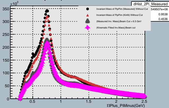
Invariant Mass of PipPim:(With/Without cut on BeamEnergy)
