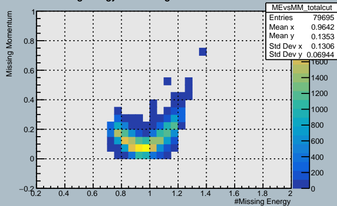
MissingEnergy vs MissingMomentum After all cut
