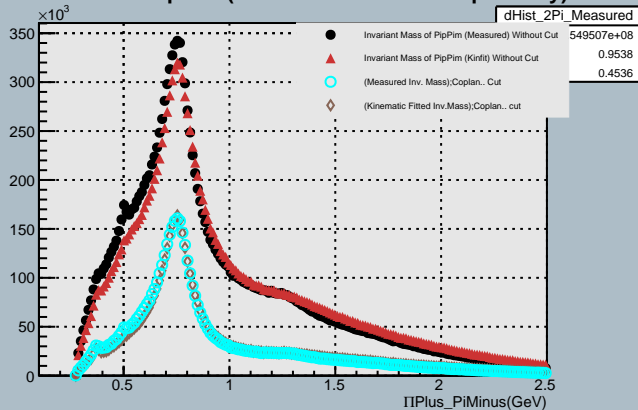
Invariant Mass of PipPim:(With/Without cut on Coplanarity)
