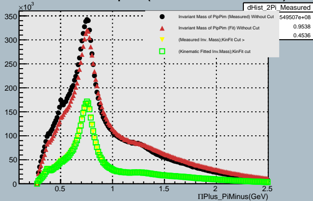
Invariant Mass of PipPim:(With/Without cut on KinFit)
