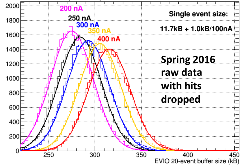
EVIO buffer size (hdl3 hit-rejected)
