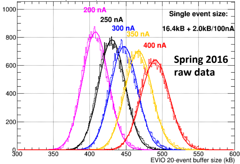
EVIO buffer size (raw data)
