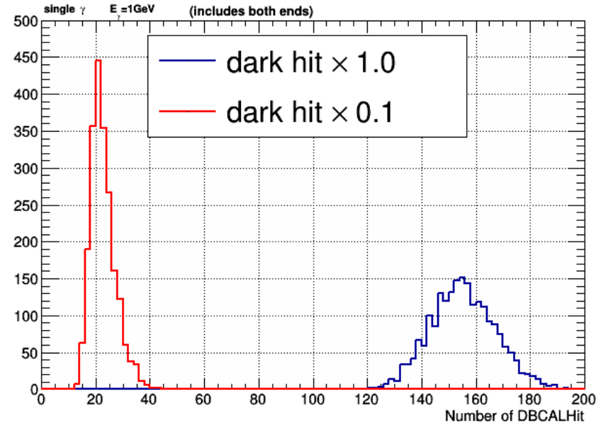
Number of Hits in BCAL
