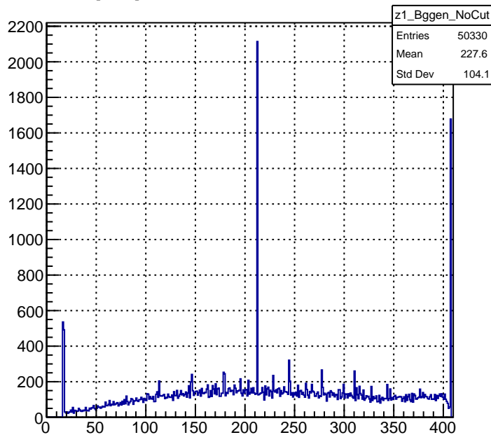
z [cms] for dNeutralParticles without cuts
