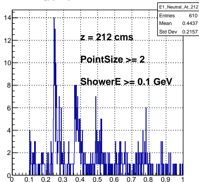
Energy [GeV] of dNeutralShowers at 212 cms
