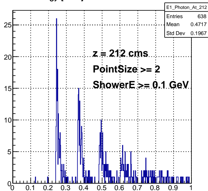
Energy [GeV] of showers at 212 cms
