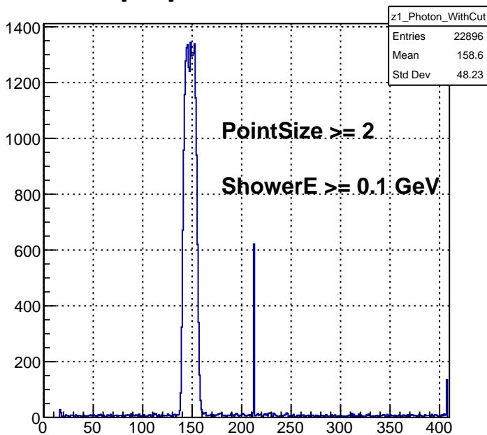
z [cms] for Photons with cuts
