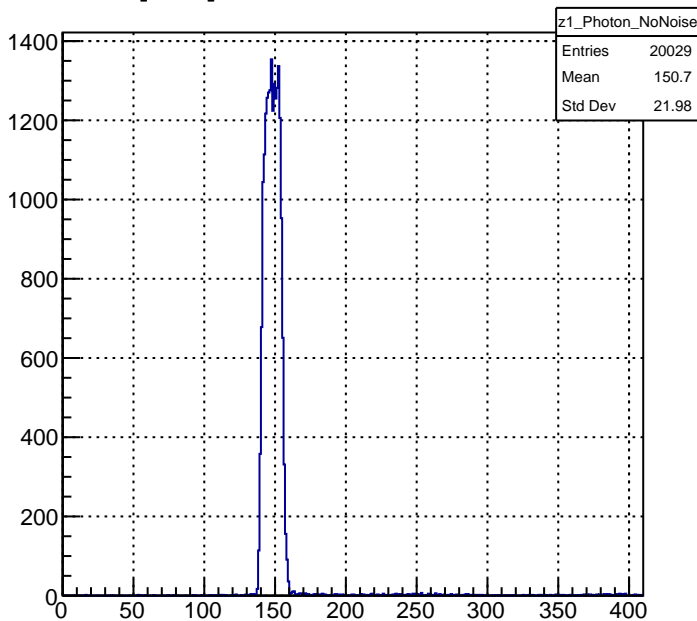
z [cms] for Photons without Noise
