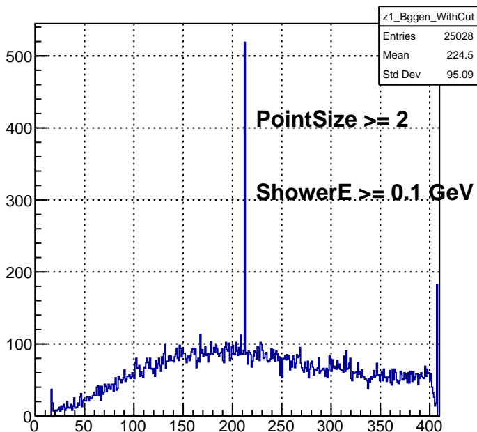
z [cms] for dNeutralParticles with cuts
