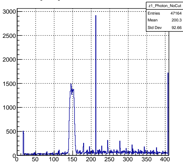
z [cms] for Photons without cuts
