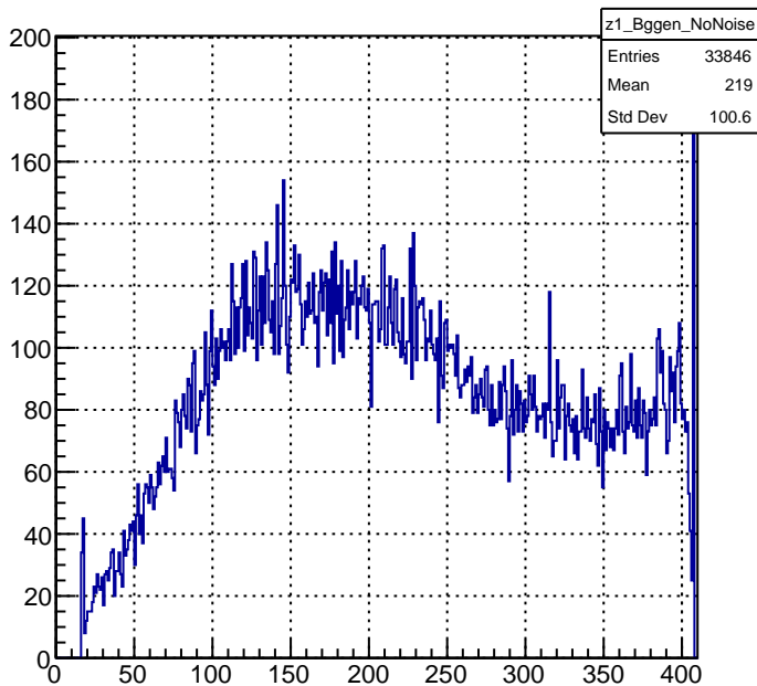
z [cms] for dNeutralParticles without Noise
