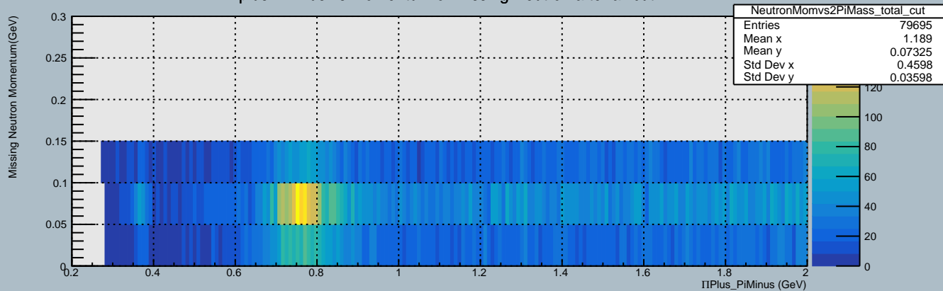
PiplusPiminus vs Momentum of Missing Neutron after all cut
