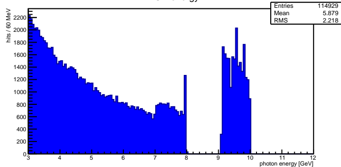
TAGH energy
