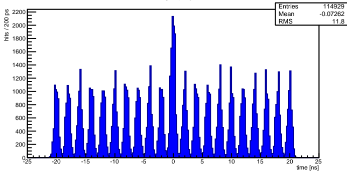
TAGH time
