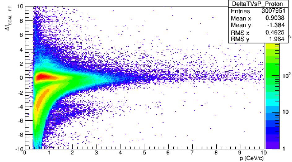
BCAL p Candidates
