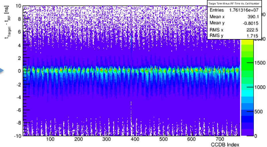
Target Time Minus RF Time Vs. Cell Number
