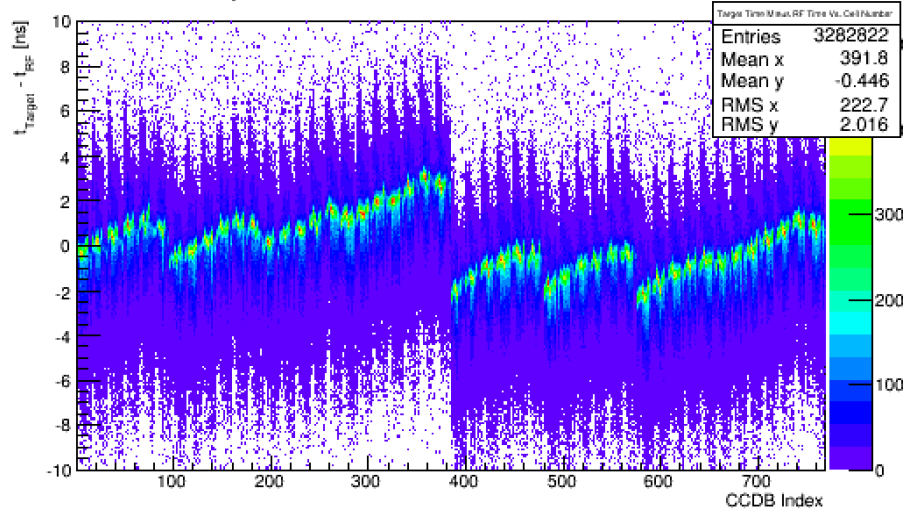
Target Time Minus RF Time Vs. Cell Number
