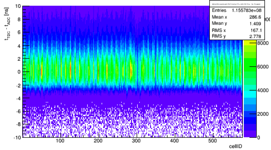
BCALHit Downstream Per Channel TDC-ADC Hit Time
