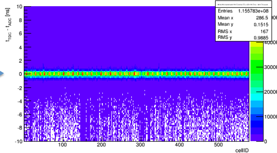
BCALHit Downstream Per Channel TDC-ADC Hit Time - TW Corrected
