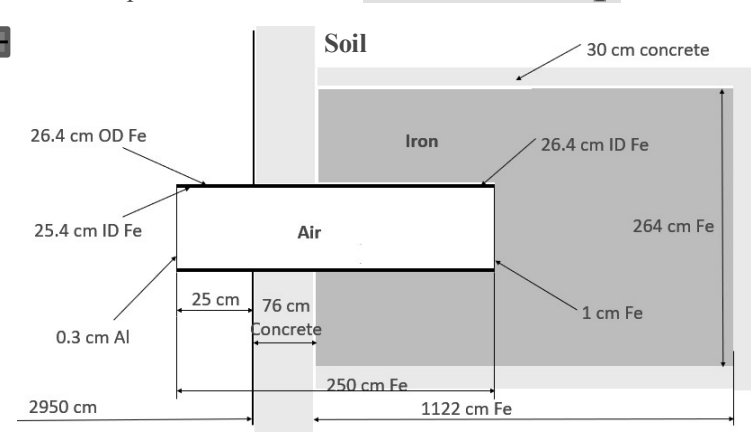
Beam dump
