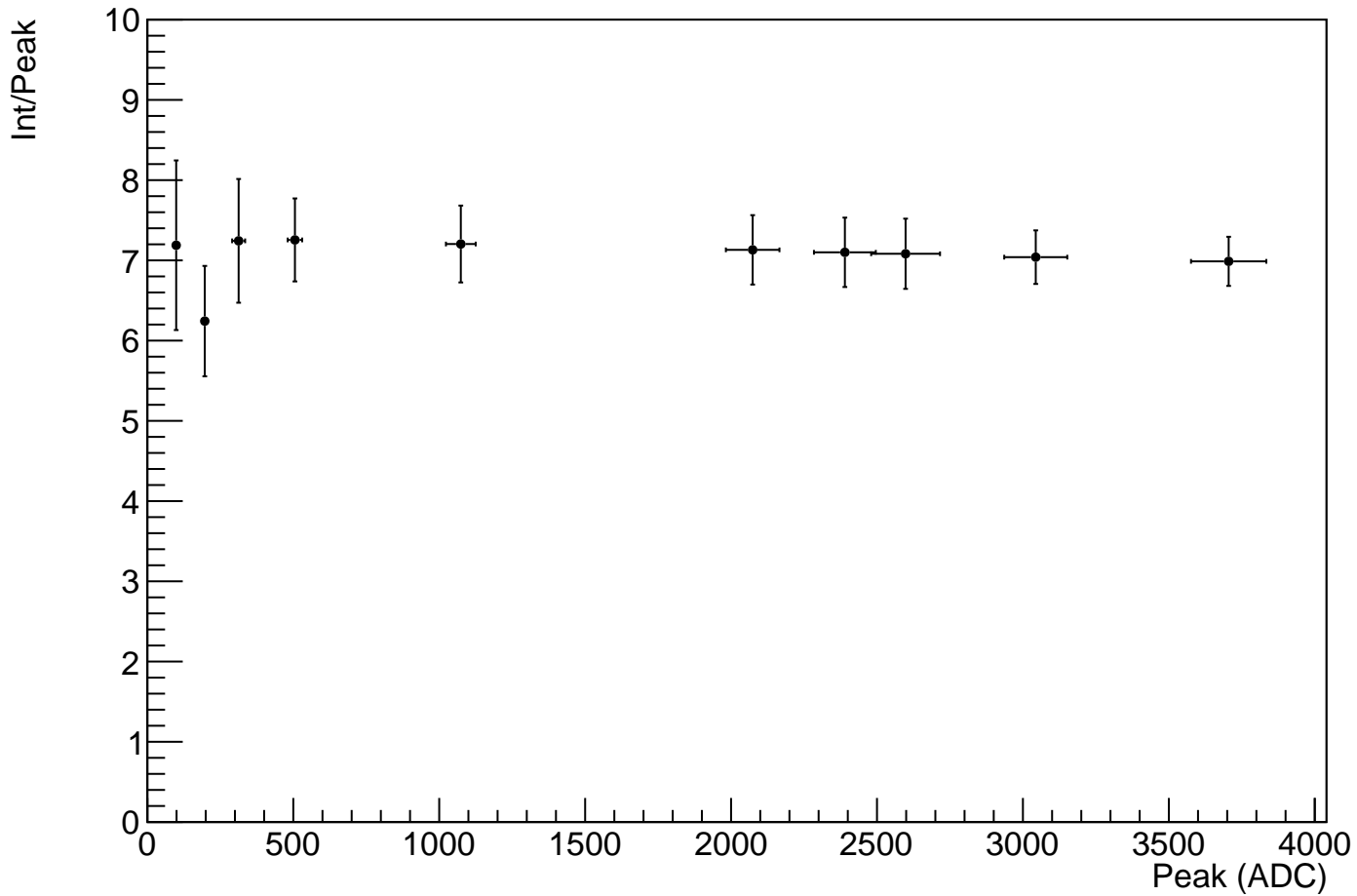
Int/Peak vs. Peak, SiPM 1
